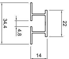
Detail Schiene Modell METRO 861
