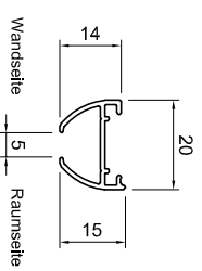
Detail Schiene Modell SPEED 460
